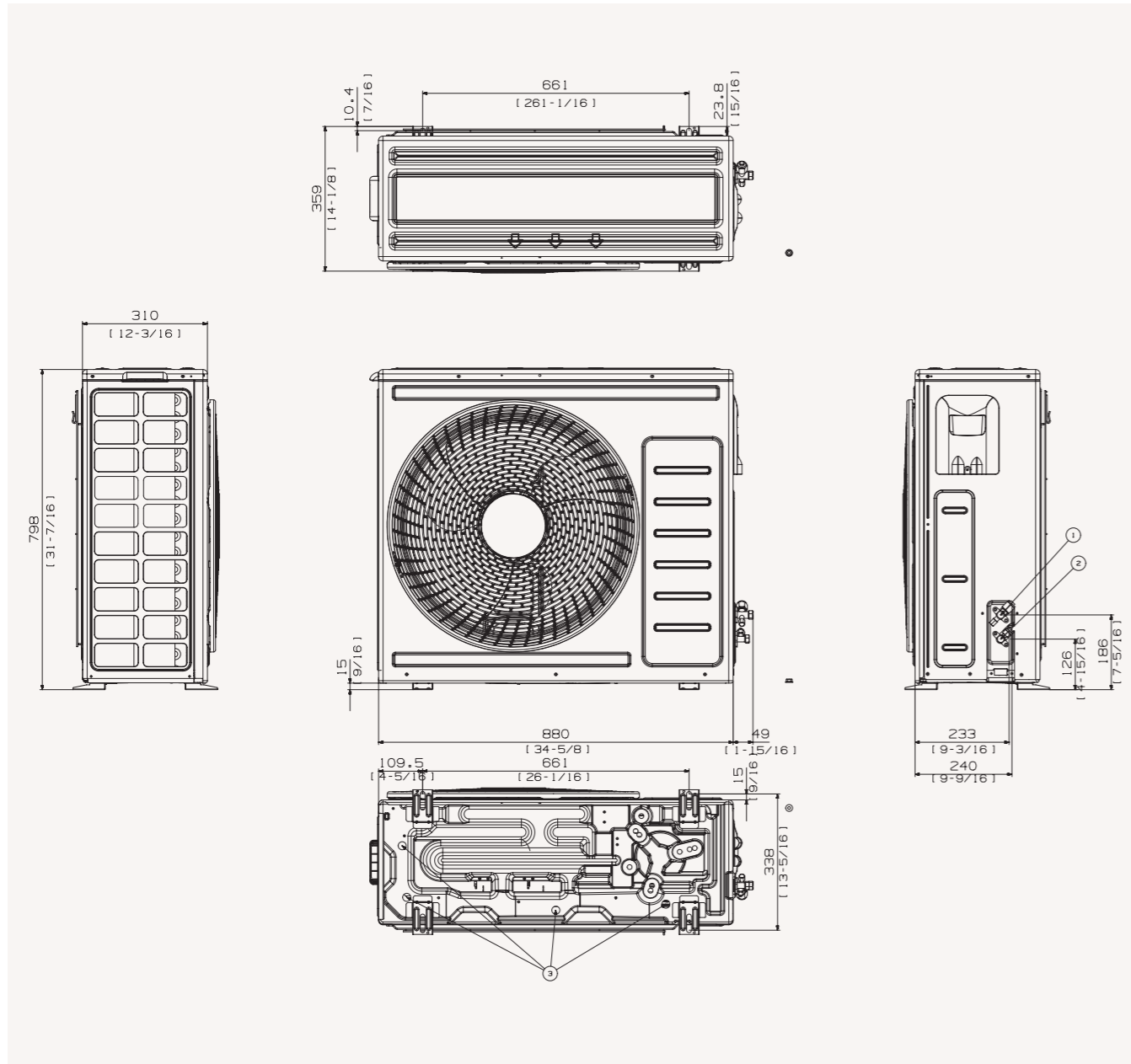
7.1 kW Outdoor Unit
