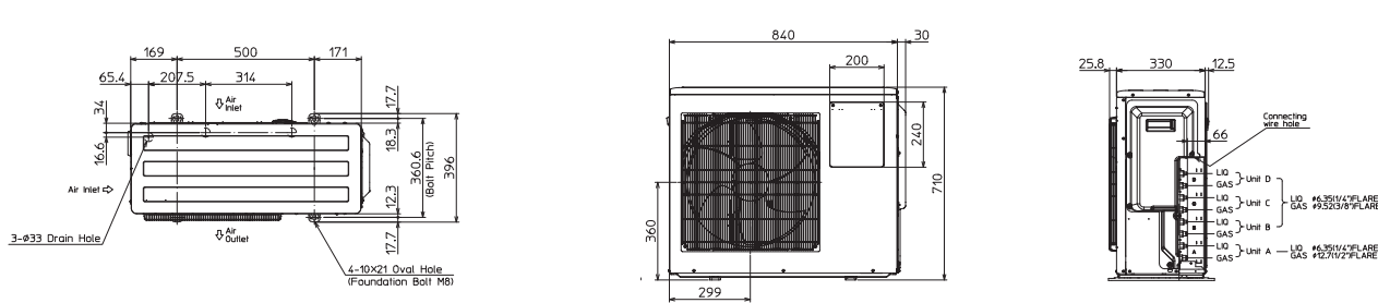
MXZ-4F72/80VF3
